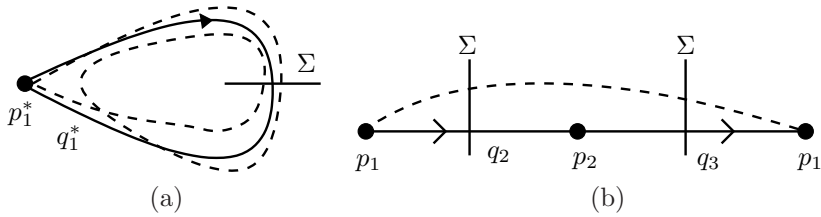
FIG. 1.1. Sketch of an itinerary for a 2-homoclinic orbit. (a) The homoclinic orbit q_1^* (solid) and its asymptotic state p_1^* at \mu = 0 , and a 2-homoclinic orbit (dashed). The Poincaré-section \Sigma is just for orientation here. (b) Schematic plot of the itinerary (solid) for a 2-homoclinic orbit (dashed) where q_2 = q_3 = q_1^* , p_1 = p_2 = p_1^* .
