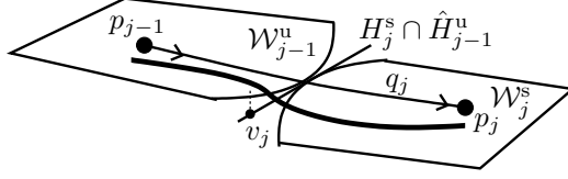
FIG. 4.3. Illustration of the notation for a tangent heteroclinic connection.
