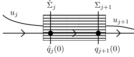
FIG. 4.2. Schematic plot of the flow box near the trajectory between \hat{q}_j(0) and q_{j+1}(0) . A left orbit u_j that enters the box at the same coordinate in \hat{\Sigma}_j as a right orbit u_{j+1} in \Sigma_{j+1} lies on the same trajectory as u_{j+1} .
