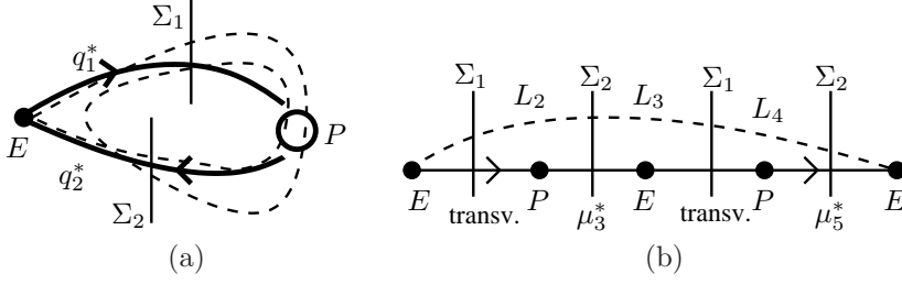
FIG. 5.2. Sketch of an itinerary for a 2-homoclinic orbit for an EP1 heteroclinic cycle. (a) the heteroclinic cycle composed of q_1^* , q_2^* (solid), and a 2-homoclinic orbit (dashed). (b) Schematic plot of the itinerary (solid) for a 2-homoclinic orbit (dashed) for which L_1 = L_5 = \infty . Note that the passing through \Sigma_1 does not generate a parameter since the heteroclinic connection from E to P is transverse. However, each passing through \Sigma_2 generates a single itinerary parameter.
