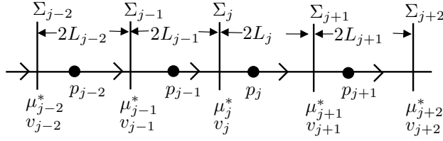
FIG. 1.2. Schematic illustration of an itinerary near index j , and the location of \mu_j^*, v_j, L_j . The arrows indicate the flow direction, connections can be copies of the same actual heteroclinic connection.
