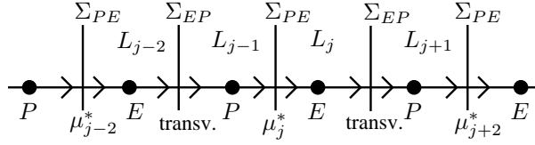
FIG. 5.1. Schematic plot of a segment of a general itinerary in an EP1 or EP2 heteroclinic cycle. Passing through \Sigma_{EP} does not require a parameter \mu_{j\pm 1} since the heteroclinic connection from E to P is transverse, but in the EP2 case a parameter v_{j\pm 1} \in \mathbb{R} appears. On the other hand, passing through \Sigma_{PE} at position j generates itinerary parameters \mu_j \in \mathbb{R}^d for the EPd case, since this connection has codimension d = 1 or d = 2 .
