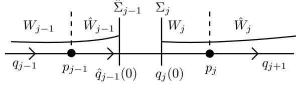
FIG. 4.1. Schematic illustration of adjacent j -variations.
