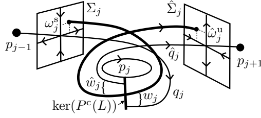
FIG. 3.1. Illustration of the notation for the flow near a periodic orbit p_j with minimal period T_j , j \in J_P . Theorem 3.2, see also Corollary 3.3, show that trajectories near \{q_j(x) : x \geq 0\} \cup \{\hat{q}_j(\hat{x}) : \hat{x} \leq 0\} are parametrised by \omega_j^s \in E_j^s(0) , \hat{\omega}_j^u \in \hat{E}_j^u(0) and L \in \{\ell T_j/2 : \ell \in \mathbb{N}, \ell T_j/2 \geq L_0\} .
