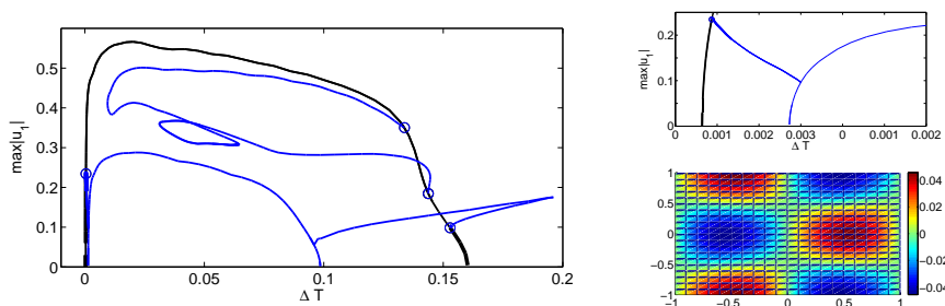
FIG. 8.4. Left panel: Bifurcation diagram as in Figure 8.3(c) with additional branches (blue) emerging from the bifurcation points of the primary branch; notably extending to \Delta T > \Delta T_2 . Right upper panel: Magnification of left panel near \Delta T = 0 . Right lower panel: u_1 -component of the small amplitude solution on the blue branch near \Delta T = 0.1 showing the wavevector k = (2, 1) .
